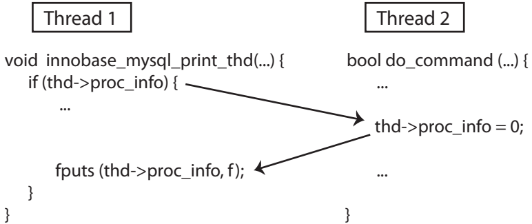
(b) MySQL #3596: Type II bug
