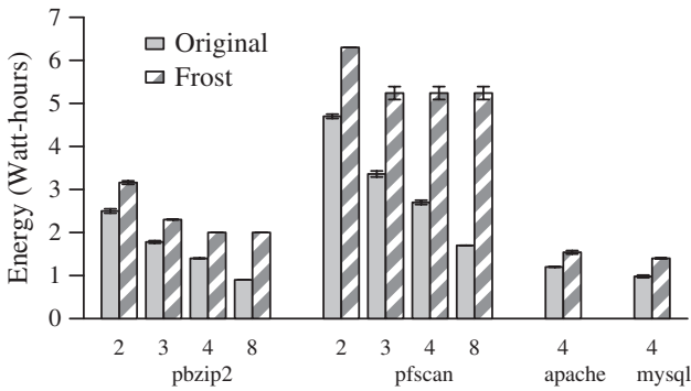
This figure shows Frost’s energy overhead. We show results for 2, 3, 4 and 8 threads for pbzip2 and pfskan, and 4 threads for Apache and MySQL. Results are the mean of five trials; error bars are 90% confidence intervals.
