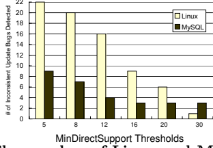
Figure 11: The number of Linux and MySQL inconsistent update bugs that are detected at different MinDirectSupport (here we use the set of bugs detected by MUVI default setting as the baseline)
