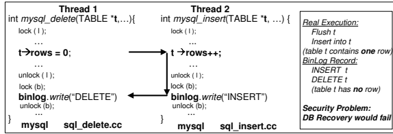
Figure 8: The false negative (bug MySQL-bug in Table 4) of Lock-set MV and Happens-before MV . The correlation between t->rows and binlog is conditional , and is therefore missed by MUVI. Specifically, t->rows can be accessed many times, and usually binlog need not be accessed together. Only when a request’s processing is at the end and t->rows is given a final value, does binlog need to be consistently modified.
