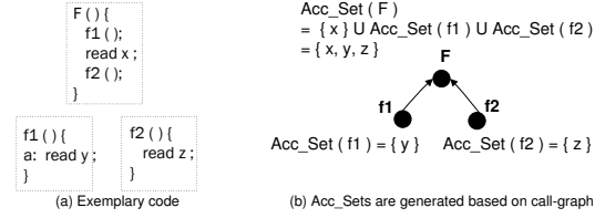
Figure 3: Acc_Set collection for an example call graph
