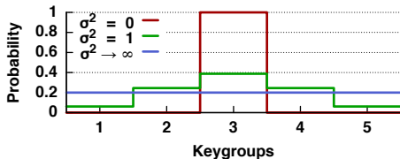
Figure 8: In our experiments, clients choose keys to access by first selecting a keygroup according to some normal distribution, then randomly selecting a key within that group according to a uniform distribution. Figure shows such a stepped normal distribution for differing variances for client #3 (of 5).
