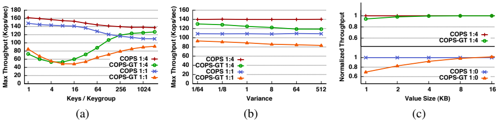
Figure 11: Maximum system throughput (using put:get ratios of 1:4, 1:1, or 1:0) for varied keys/keygroup, variances, and value sizes.
