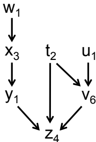
Figure 6: A sample graph of causal dependencies for a client context. Arrows indicate causal relationships (e.g., x_3 depends on w_1 ). The table lists all dependencies for each value and the “nearest” dependencies used to minimize dependency checks.
