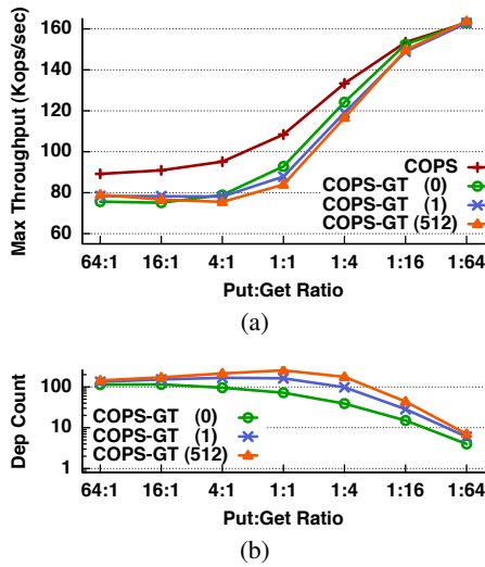
Figure 10: Maximum throughput and the resulting average dependency size of COPS and COPS-GT for a given put:get ratio. The legend gives the variance (i.e., 0, 1, or 512).
