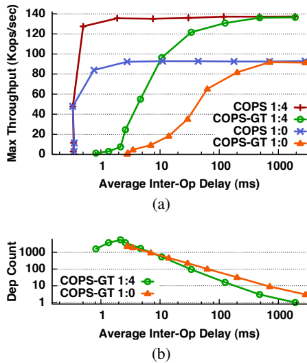
Figure 9: Maximum throughput and the resulting average dependency size of COPS and COPS-GT for a given inter-put delay between consecutive operations by the same logical client. The legend gives the put:get ratio (i.e., 1:0 or 1:4).
