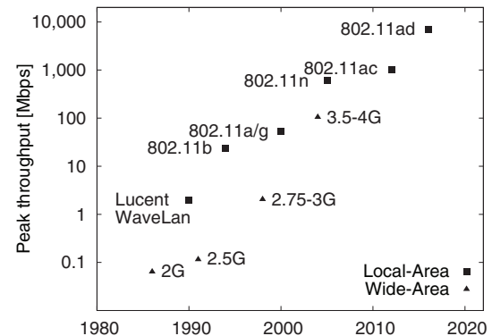
Figure 1: Peak throughput of local-area and wide-area networks for the past three decades; y-axis is log scale.
